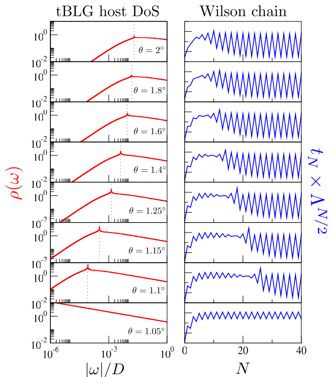
FIG. 7: Left panels: DoS used in our NRG calculations, obtained from analysis of the effective BM model, for different twist angles \theta as used in the main text. Vertical dotted lines show the E_v scale at which the vHs divergence occurs. This scale moves to lower energies as the magic angle is approached. Right panels: corresponding Wilson chain coefficients.
