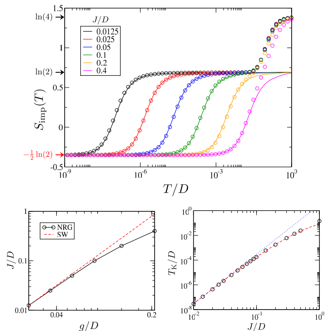
FIG. 6: NRG results for an impurity embedded in magic angle TBG. Main panel: Entropy S_{\text{imp}} vs T for Anderson and Kondo impurities (points and lines respectively) for different impurity-host couplings. For a given Kondo J , the low temperature physics of an Anderson model with fixed U = 0.4D is fit by tuning g . The relationship between J and g is shown in the lower-left inset (points), comparing with the SW result (red dashed line). The evolution of T_K with J is shown in the lower-right inset (points), comparing with Eq. 25 (red dashed line) and its small- J asymptote (blue dotted line). T_K is extracted numerically from NRG results for the entropy, defined in practice via S_{\text{imp}}(T = T_K) = 0 .
