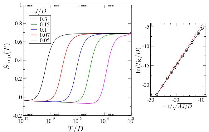
FIG. 8: Main panel: NRG results for the impurity entropy S_{\text{imp}} vs temperature T for different bare coupling strengths J , in a system with a pure log-diverging DoS (standard vHs). Right inset shows the extracted T_K scale (points), compared with Eq. 24 (black line) and the asymptotic result T_K \sim D e^{-1/\sqrt{AJ/D}} (red dashed line), with A = a\rho_0 D/2 .
