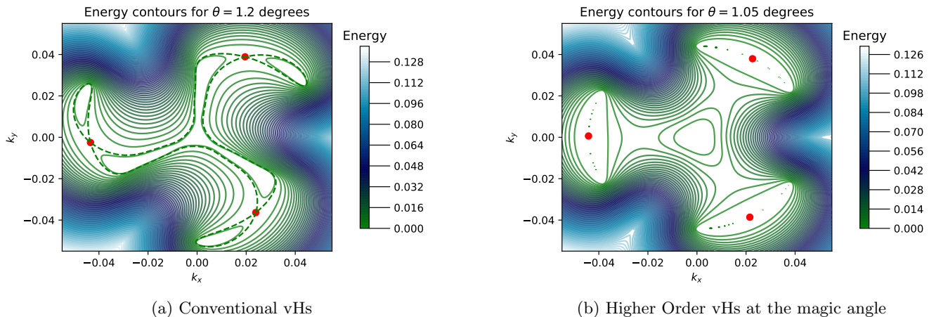
FIG. 2: Low-energy features of the particle-hole symmetric BM model of pristine TBG, showing energy contours of the dispersion \varepsilon(\mathbf{k}) as a function of momentum \mathbf{k} in the extended MBZ. Red points show the saddle points of the dispersion, corresponding to the van Hove singularities. Dashed lines show the contours at energy E_v , on which the van Hove points sit.
